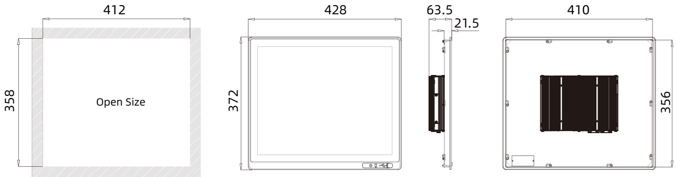
Panel Cutout Dimensions: 412 x 358mm ( 16.22 x 14.09in )
