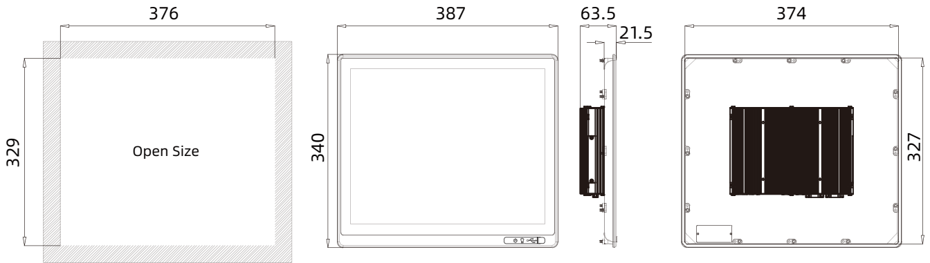
Panel Cutout Dimensions: 376 x 329mm ( 14.80 x 12.95in)
